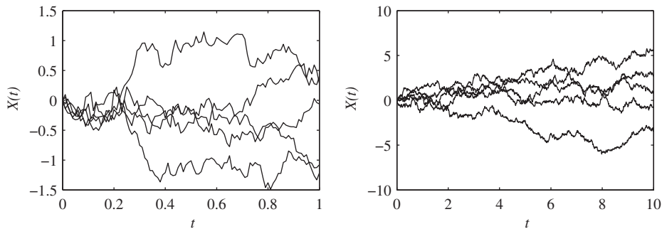
Figure 13.7 Sample paths of Brownian motion.
