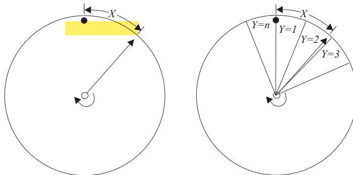
Figure 4.1 The random pointer on disk of circumference 1.
